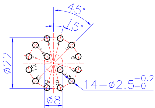
P.C.B MOUNTING HOLE
