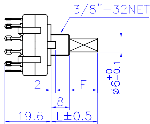
DETAIL OF TERMINAL
